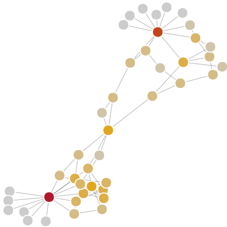
Degree
