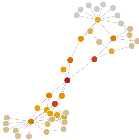
Closeness
