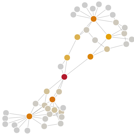
Betweenness
