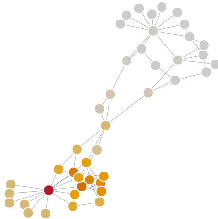
Eigenvector
