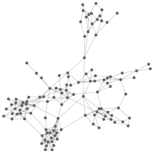
Stochastic block model network
