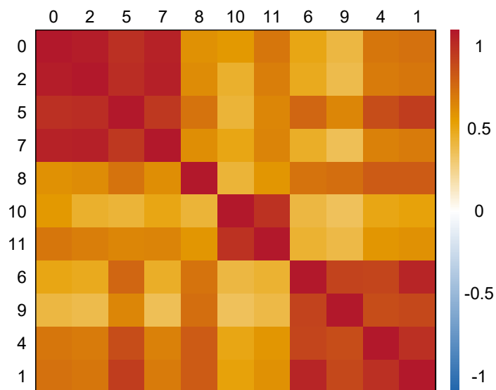
Stochastic block model GCM
