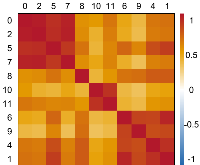
Barabasi-Albert GCM
