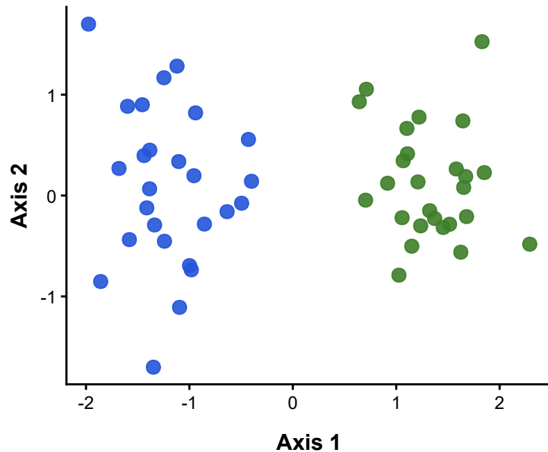
Ordination of sample distances
