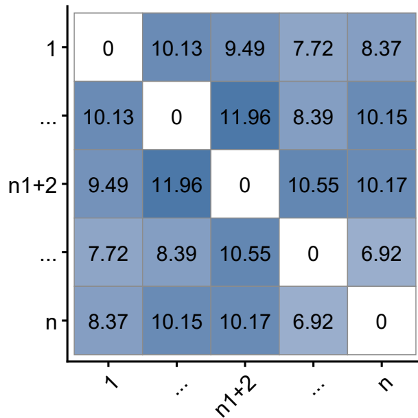
Between-sample diversity
