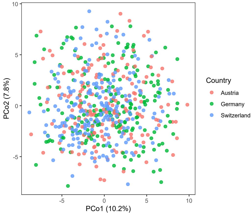
Euclidean distance after multRepl + CLR: Country
