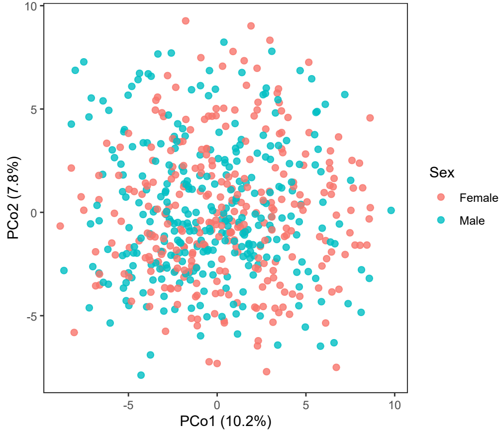
Euclidean distance after multRepl + CLR: Sex
