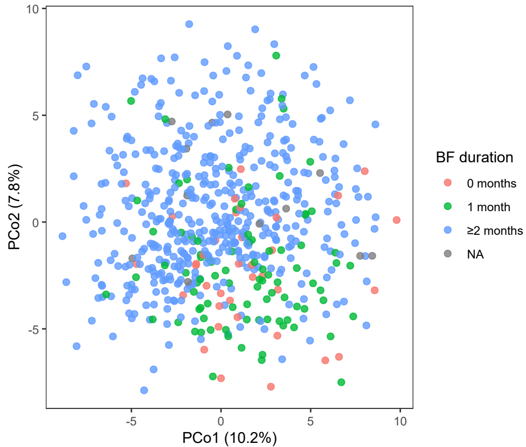
Euclidean distance after multRepl + CLR: BF duration
