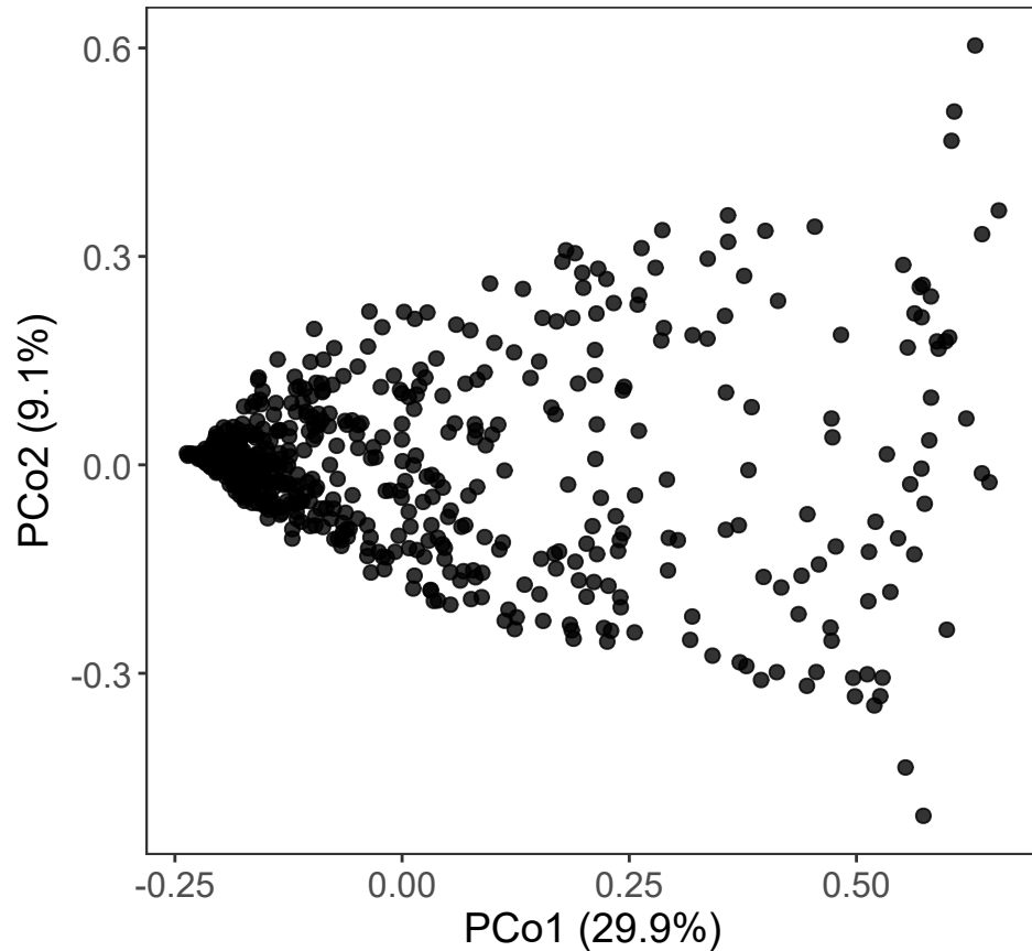
Bray-Curtis dissimilarity
