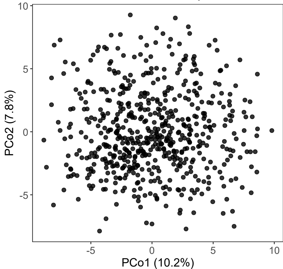
Euclidean distance after multRepl + CLR
