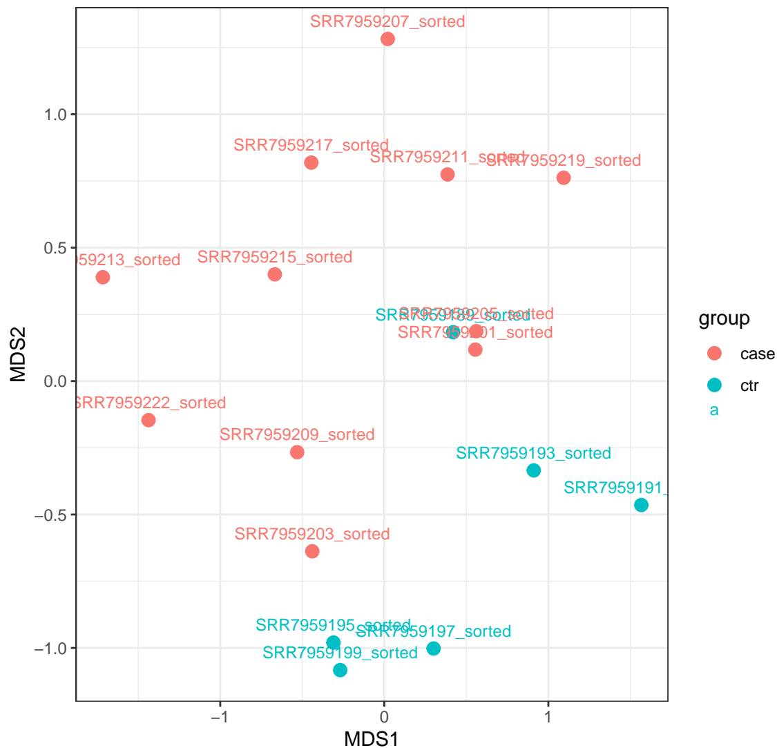
example – MDS plot
