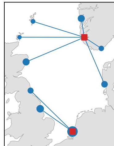
(f) Capacitated FLP, single sourcing
