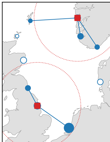
(e) Uncapacitated FLP
