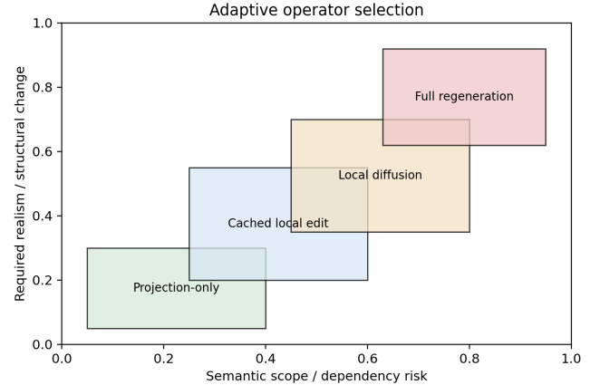
Figure 2: Conceptual operator selection space. Simple local edits favor deterministic projection or cached local rendering, while structurally broad edits may require full regeneration.
