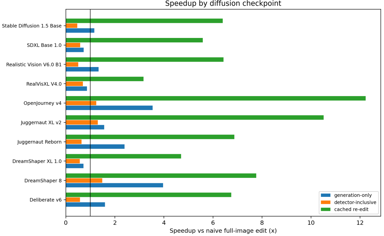
Figure 4: Speedup by model. The generation-only metric isolates local rendering cost; the detector-inclusive metric represents first-edit user latency; cached re-edit represents repeated semantic layer editing.
