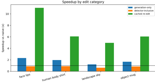
Figure 3: Speedup by edit category. Cached semantic re-edit is positive for all categories, while detector-inclusive first-edit speedup is below 1x on average.
