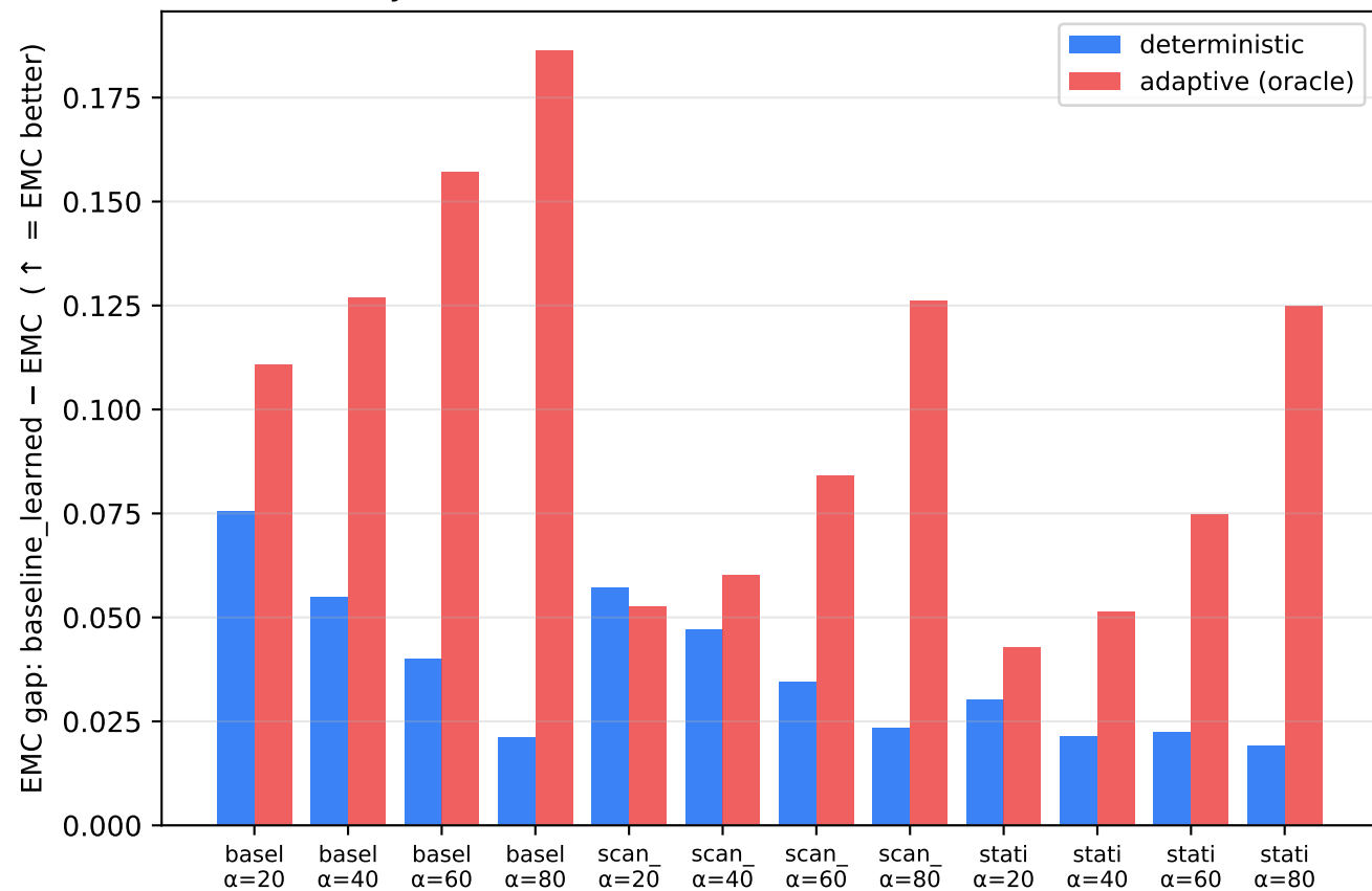
Synthetic benchmark (12 conditions, default32)
