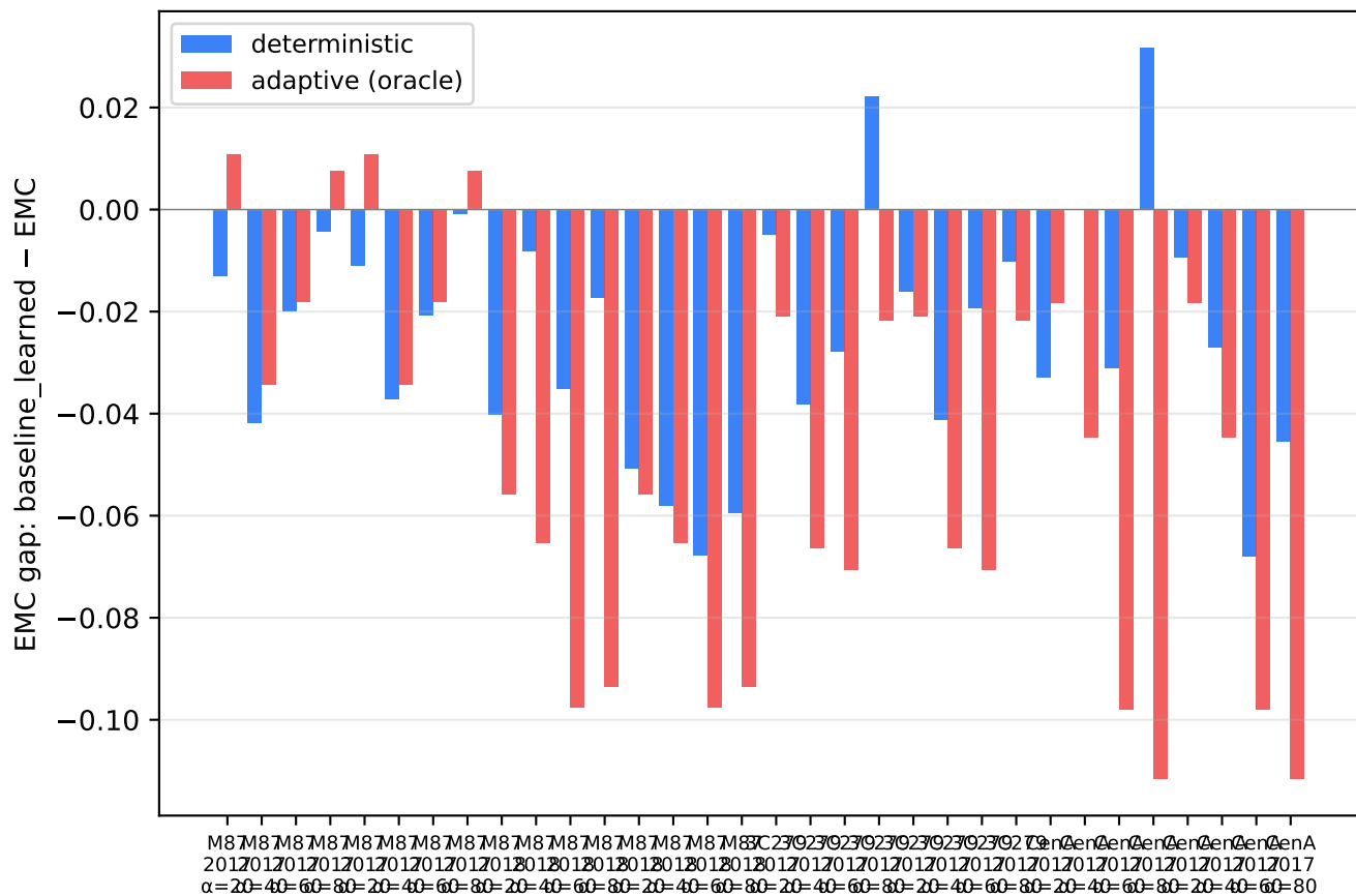
Public EHT (4 releases \times 2 families \times 4 sf = 32 conditions)
