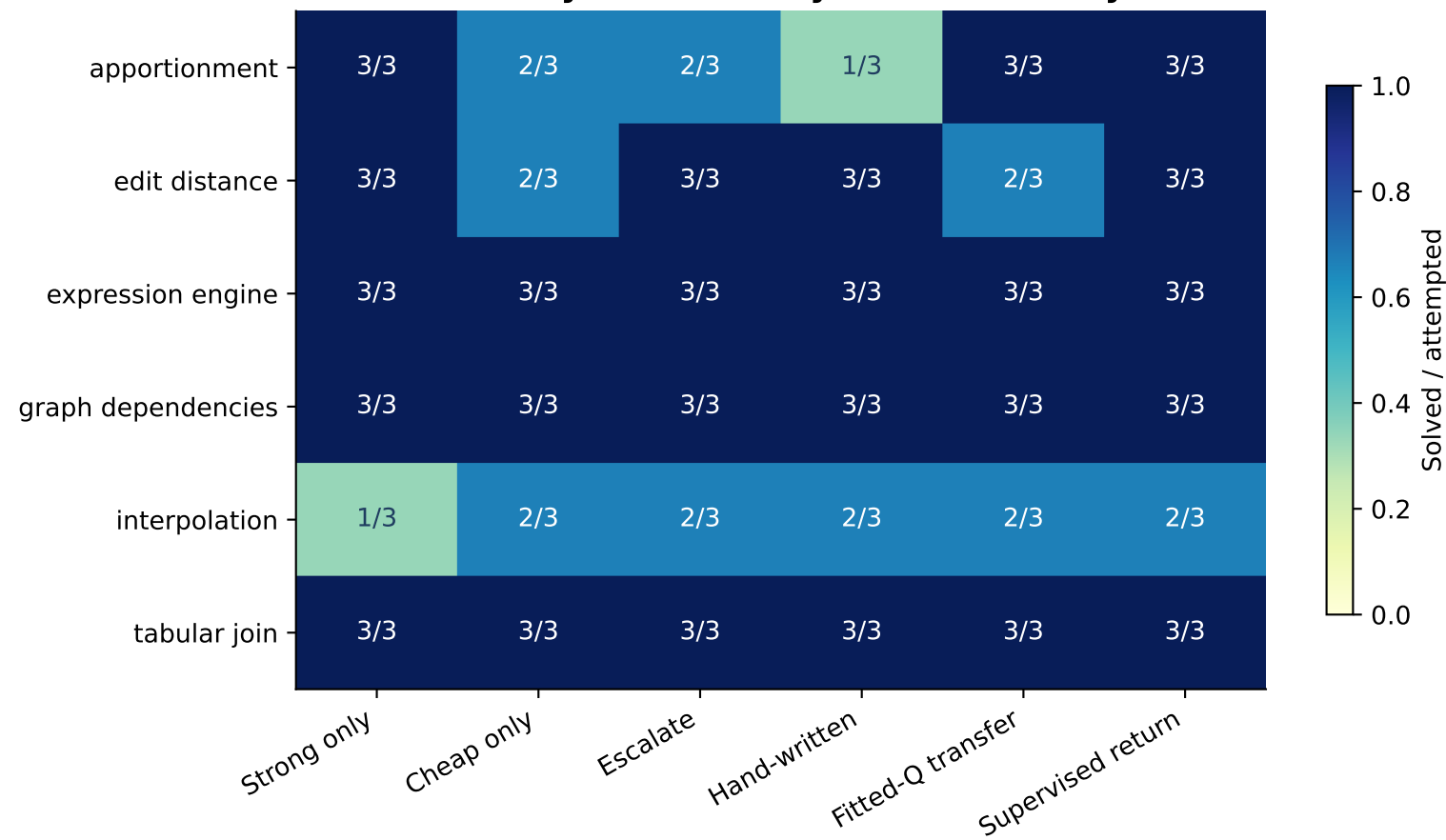
Primary outcomes by held-out family
