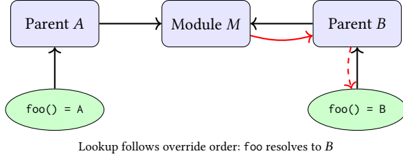
Figure 4. Symbol resolution in a Merkle-based inheritance graph. Module M inherits from parents A and B , with left-to-right override precedence. The red arrows illustrate the path taken to resolve the symbol foo , which is found in B . Dotted red arrows represent resolution from the parent to the symbol definition.
