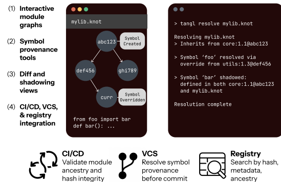
Figure 7. A conceptual overview of developer tooling for Merkle-based module systems. IDE and CLI tools provide layered insights: (1) interactive module graphs show lexical and resolved ancestry; (2) symbol provenance tools trace resolution across override chains; (3) diff and shadowing views visualize active vs overridden definitions; and (4) integration with CI/CD, VCS, and registries supports reproducibility and ecosystem interoperability.
