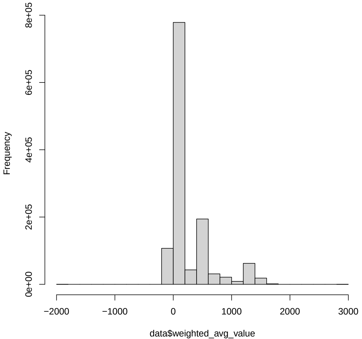
Histogram of data$weighted_avg_value
