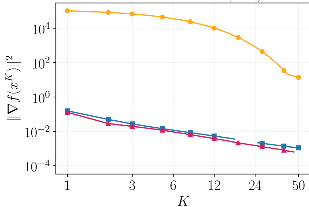
Gradient Descent (GD)
