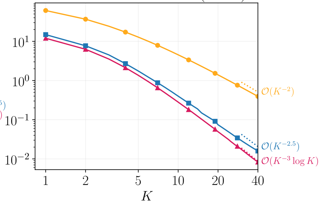
Fast Gradient Method (FGM)
