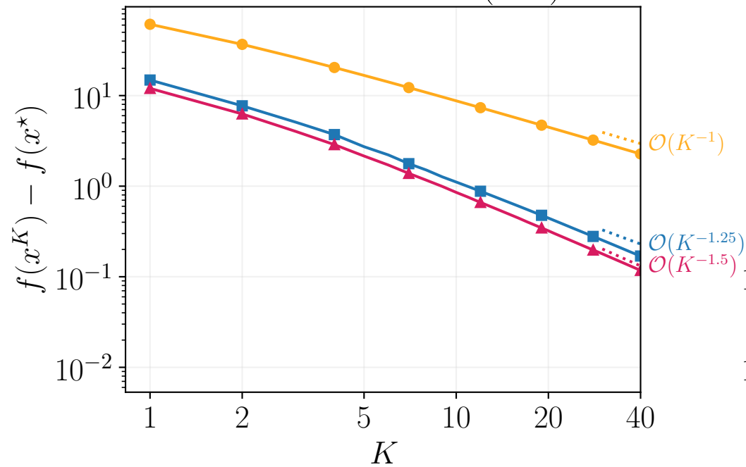
Gradient Descent (GD)
