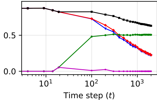
In-sample objective value
