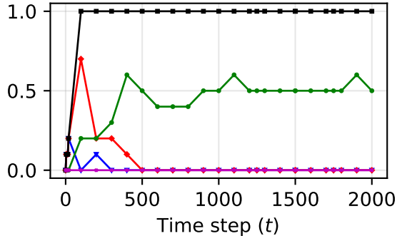
Confidence 1 - \hat{\beta}_t
