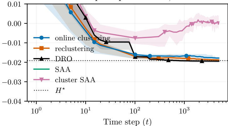
Out-of-sample expected value, K = 15
