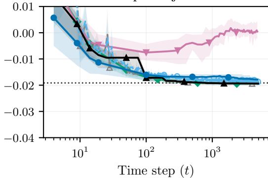
Out-of-sample objective value
