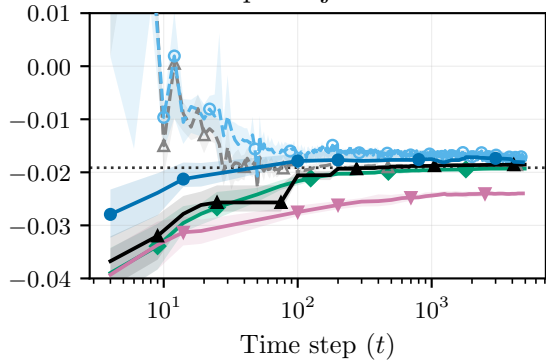
In-sample objective value
