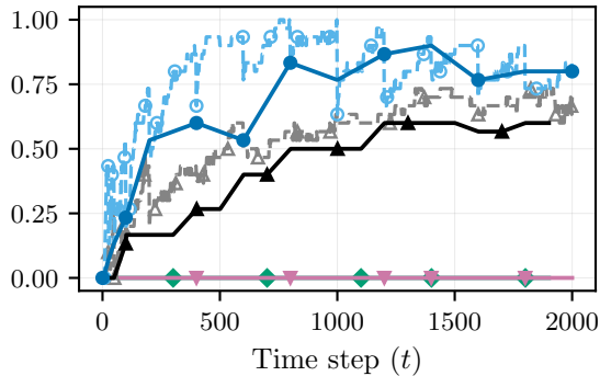
Confidence 1 - \hat{\beta}_t
