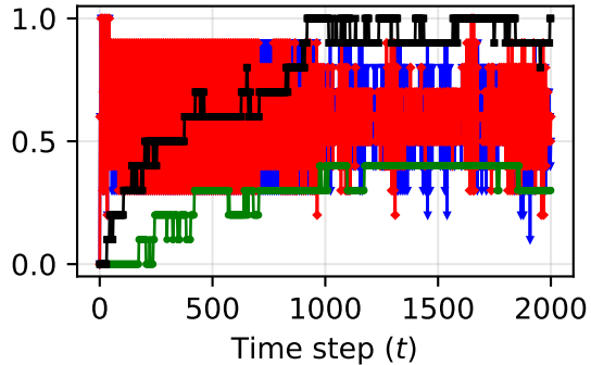
Confidence 1 - \hat{\beta}_t
