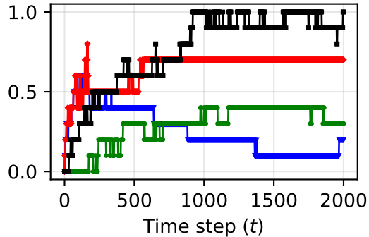
Confidence 1 - \hat{\beta}_t
