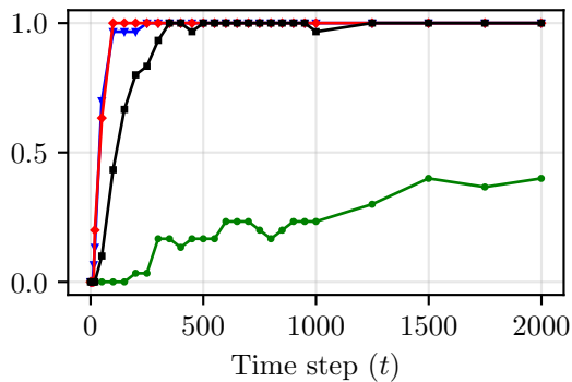
Confidence 1 - \hat{\beta}_t
