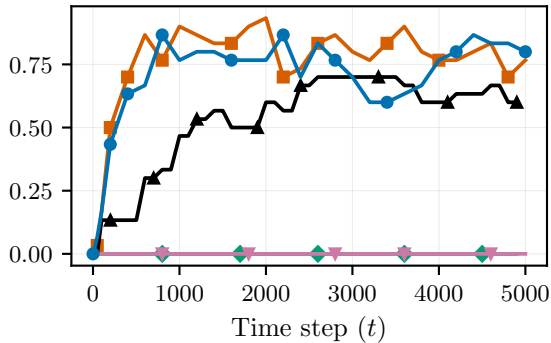
Confidence 1 - \hat{\beta}_t
