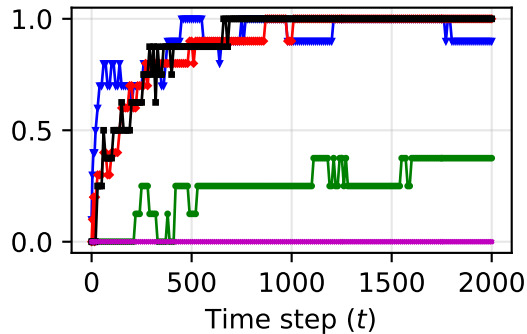
Confidence 1 - \hat{\beta}_t
