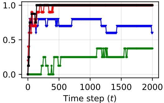
Confidence 1 - \hat{\beta}_t
