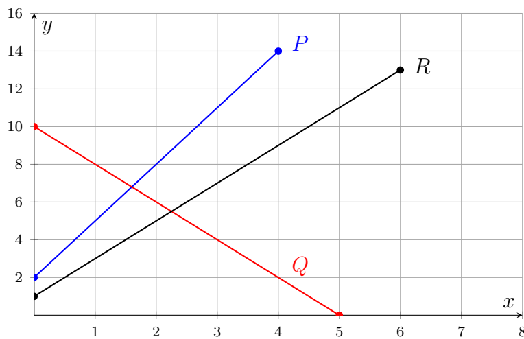
Graph Bank
