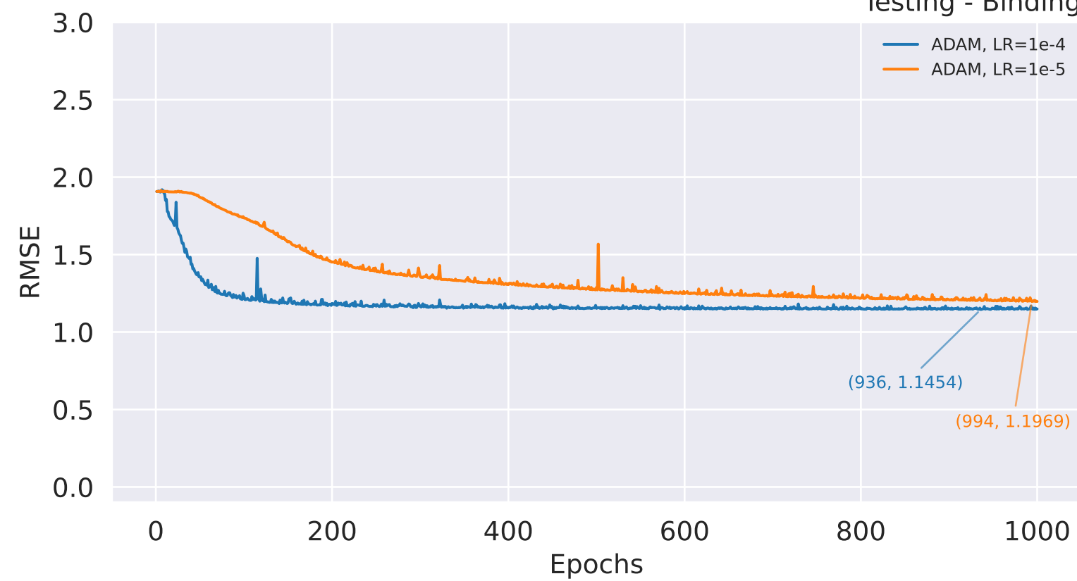
Testing - Binding
