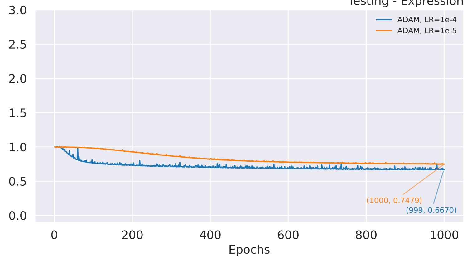
Testing - Expression
