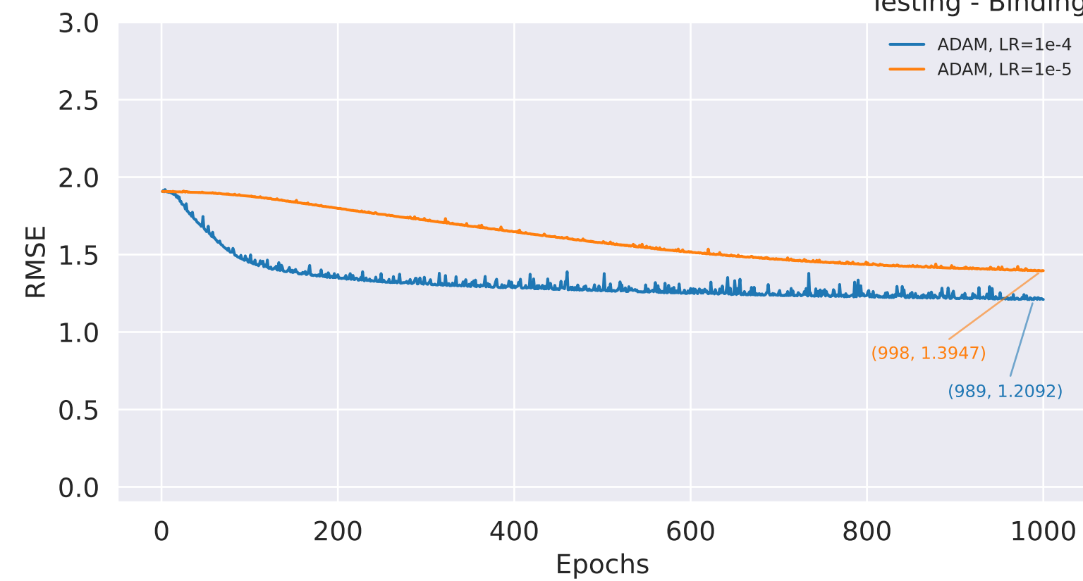
Testing - Binding
