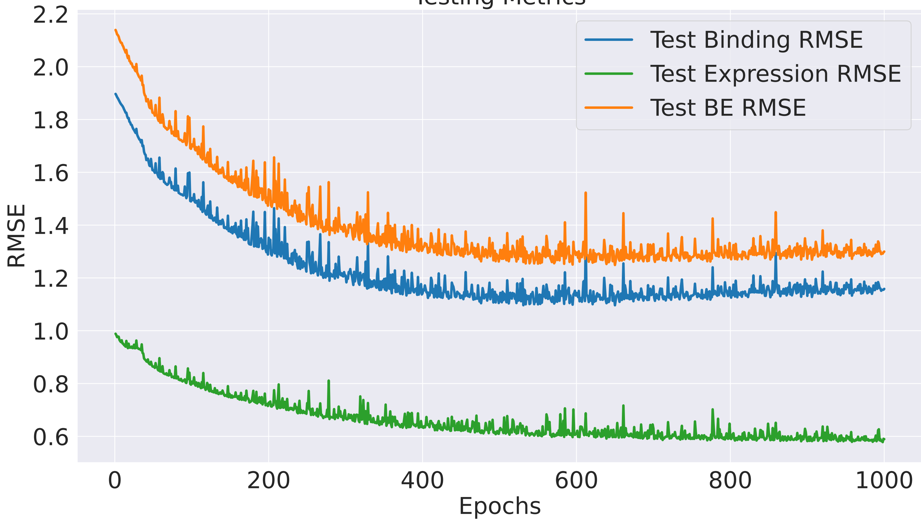
Testing Metrics
