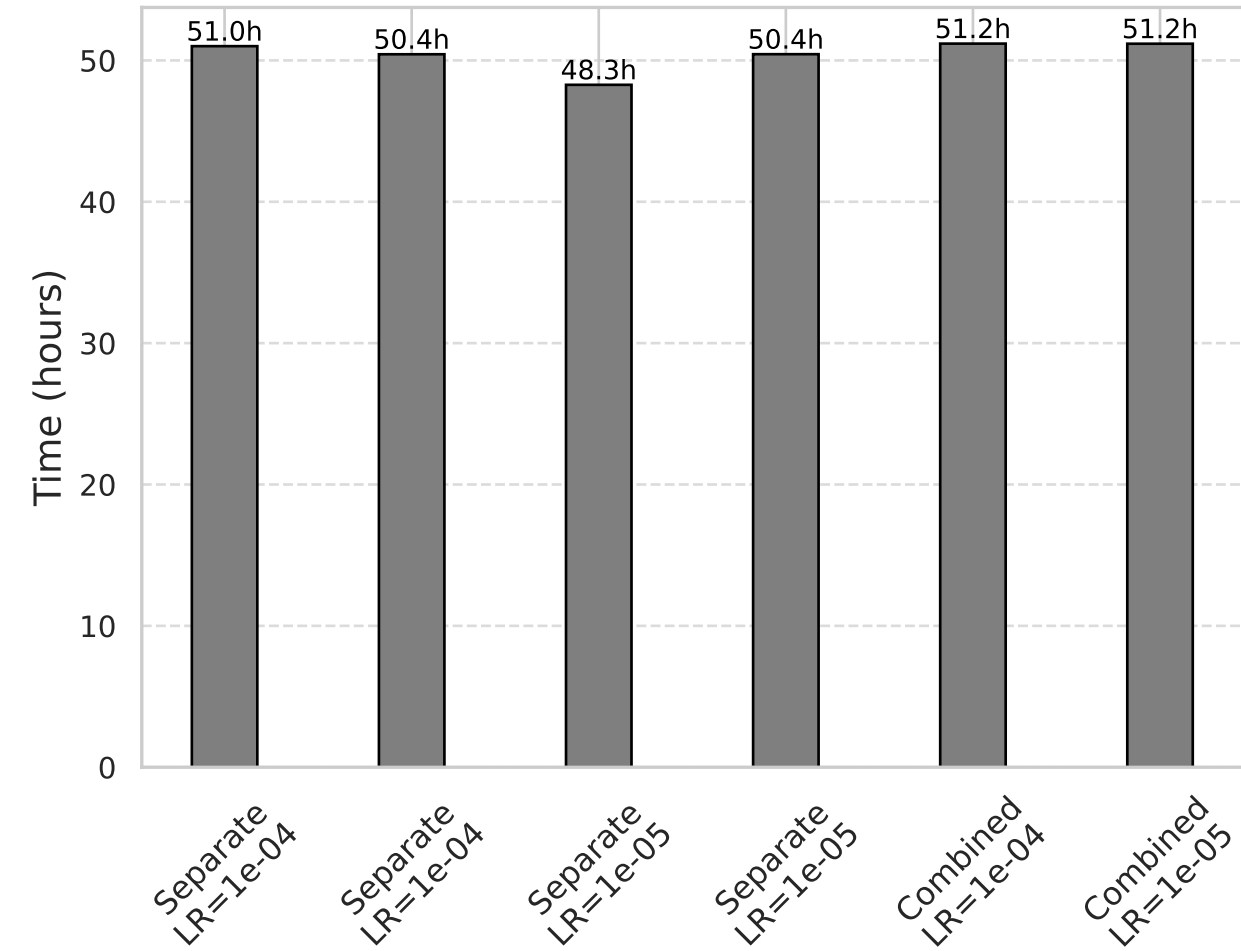
Runtime
