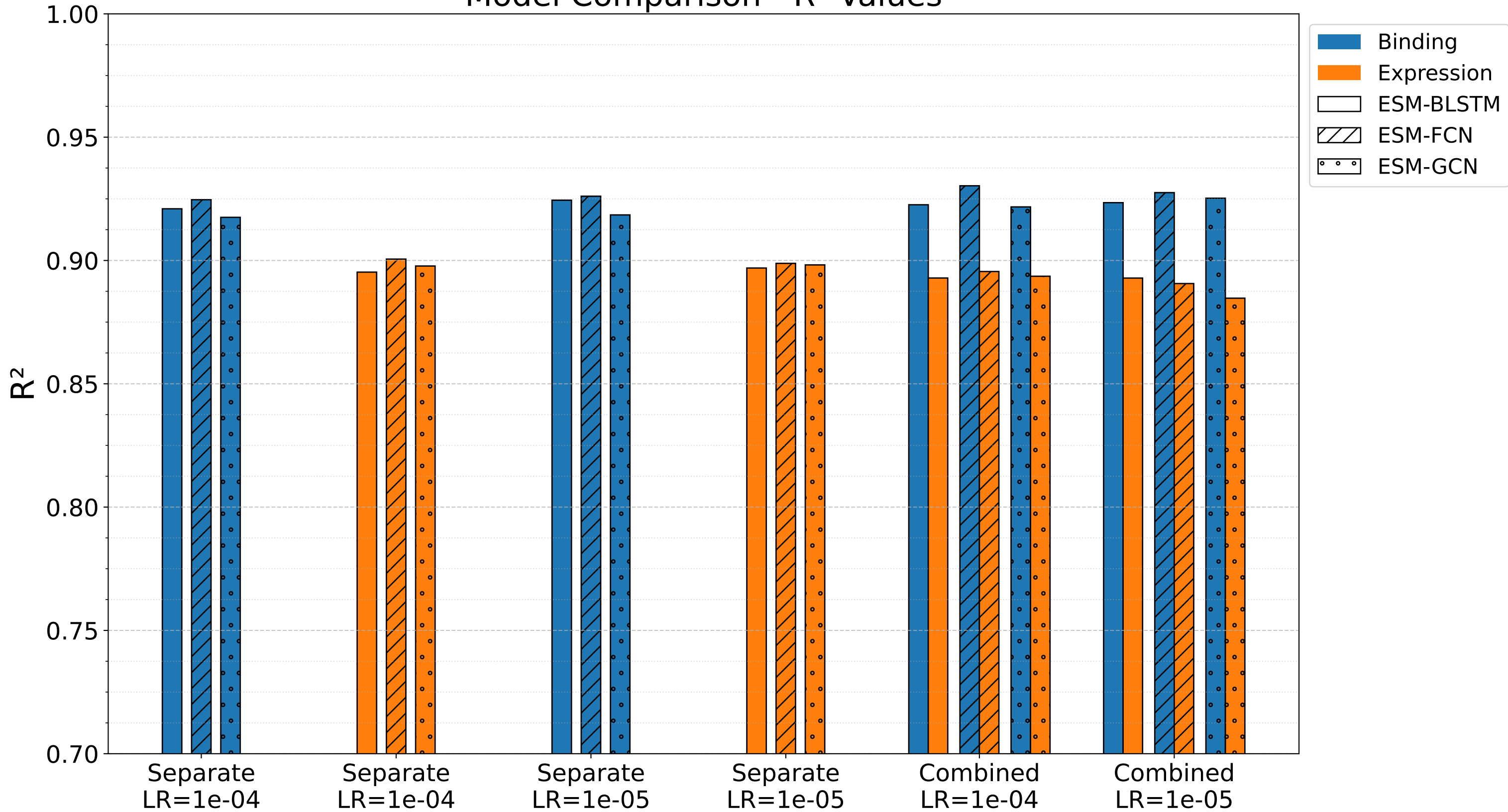
Model Comparison - R 2 Values
