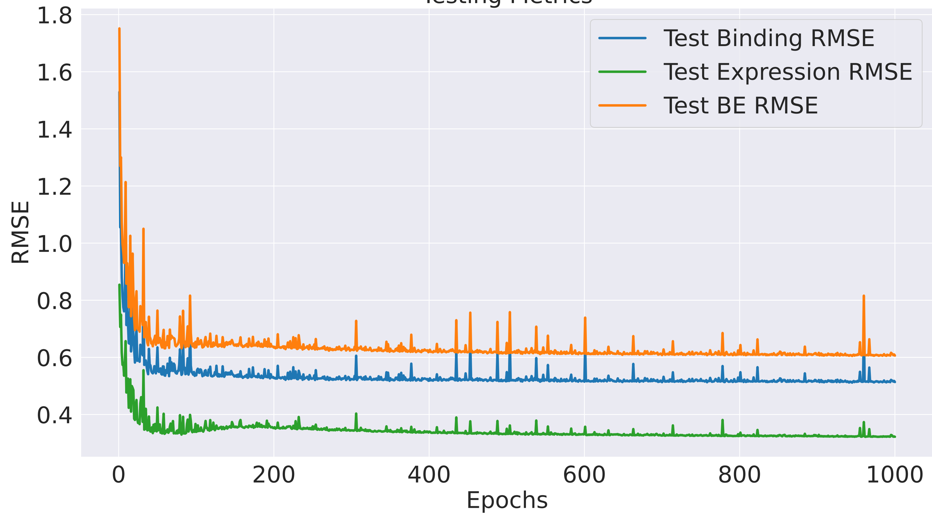
Testing Metrics
