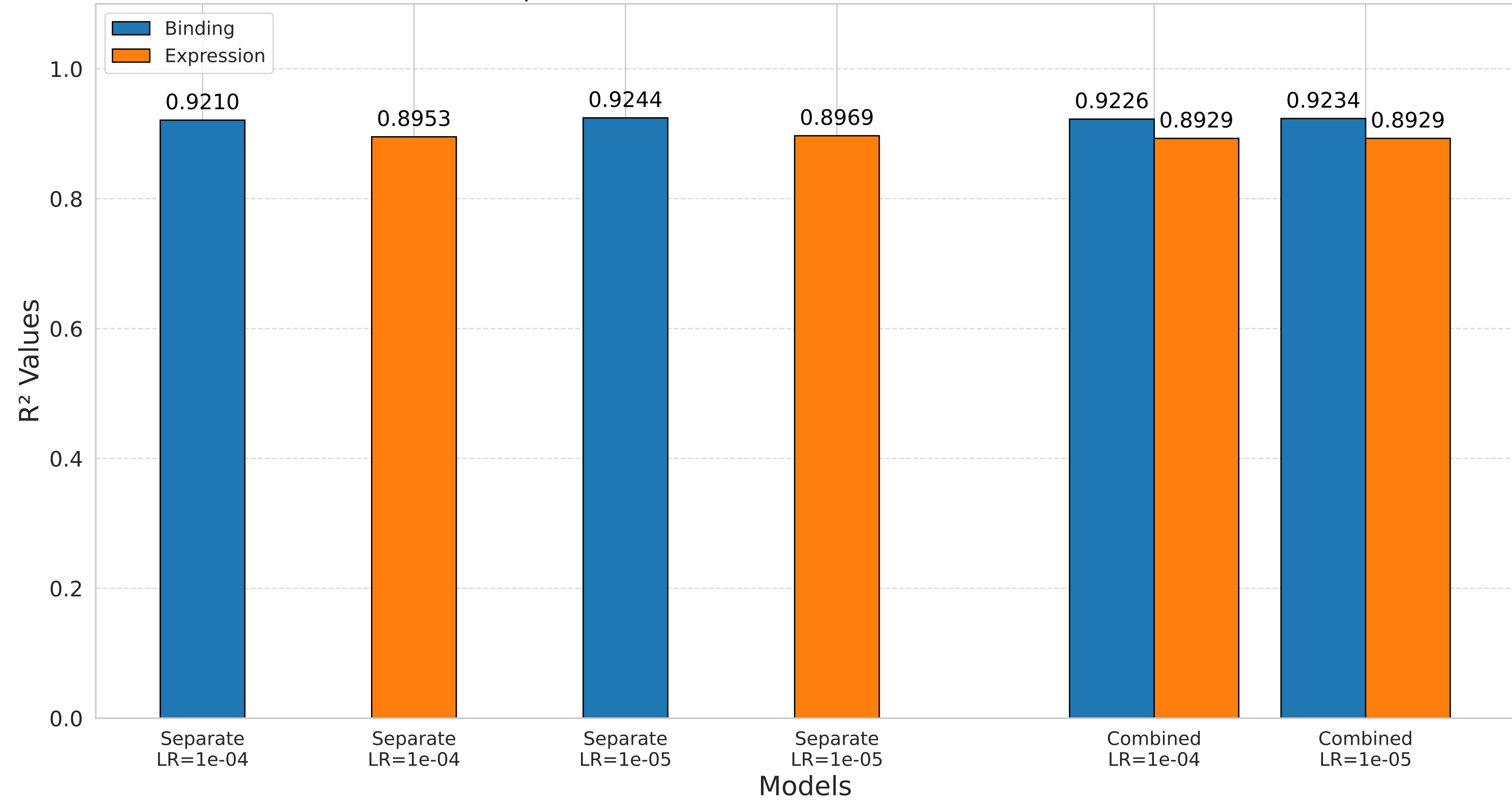
Comparison of R 2 Values Across ESM-BLSTM Models
