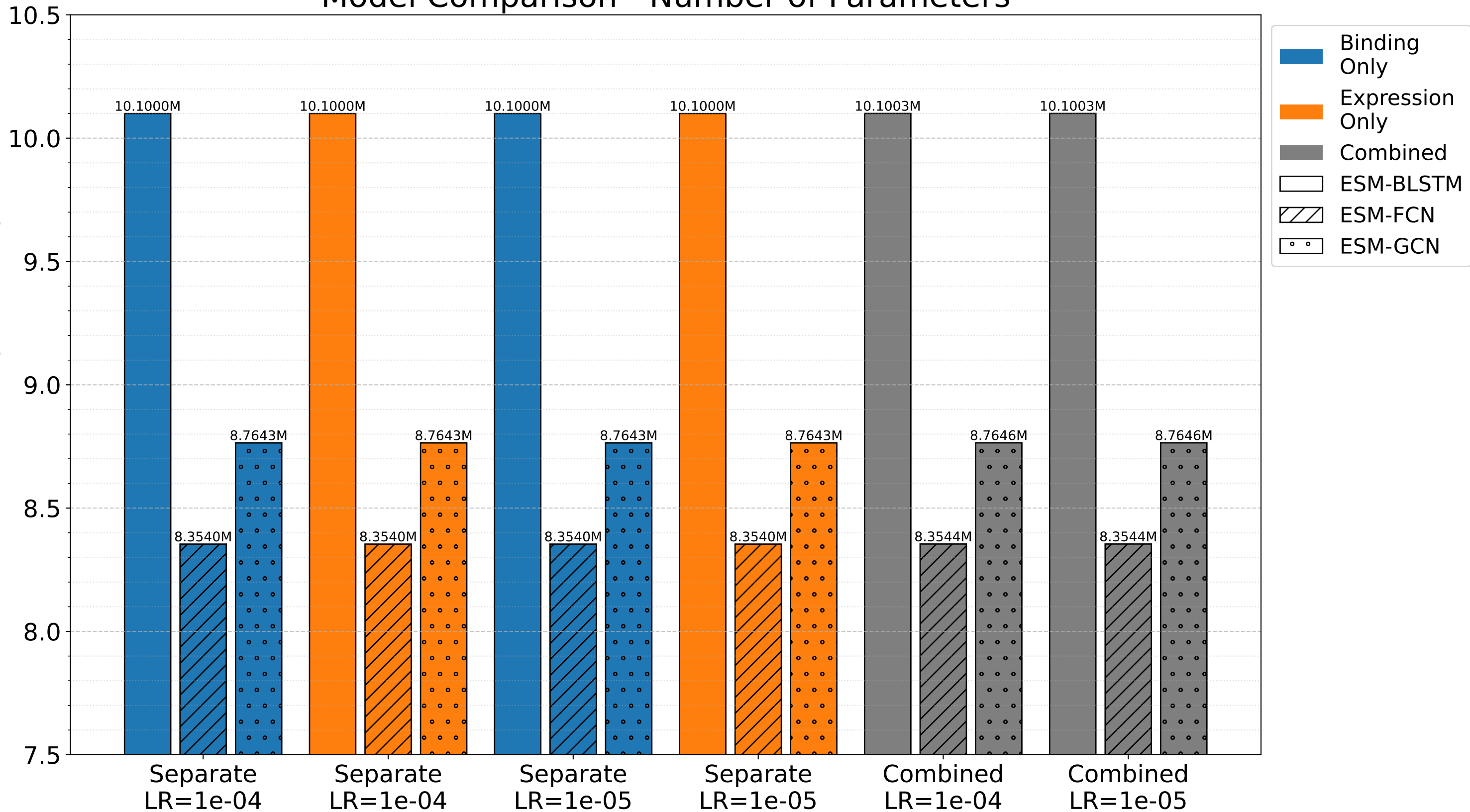
Model Comparison - Number of Parameters
