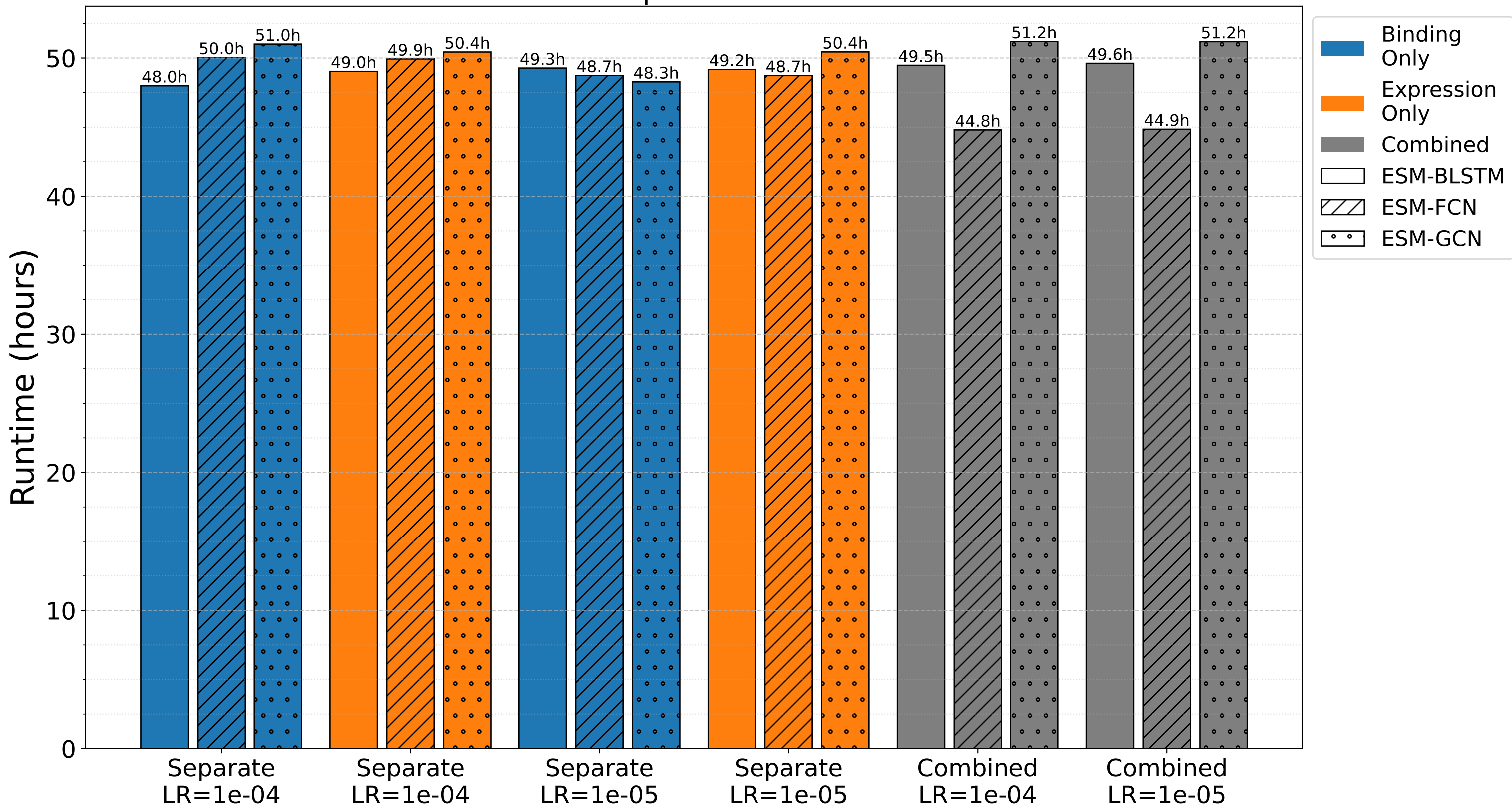
Model Comparison - Runtime
