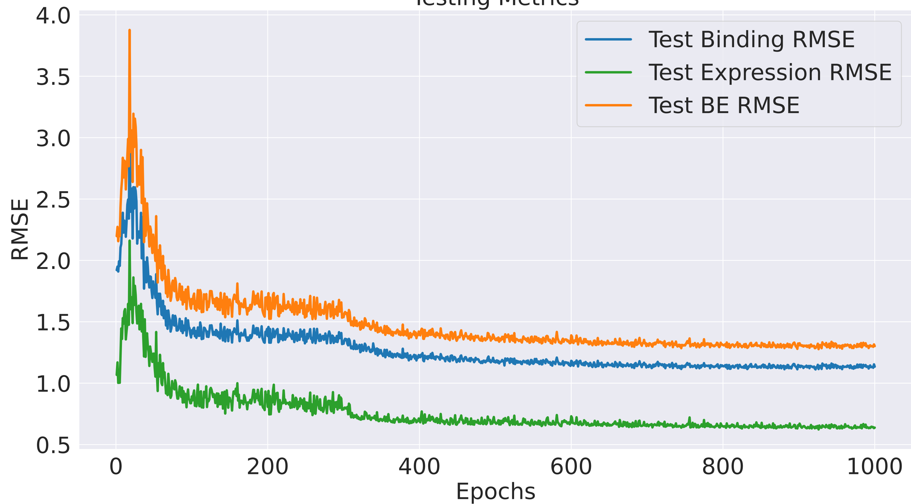
Testing Metrics
