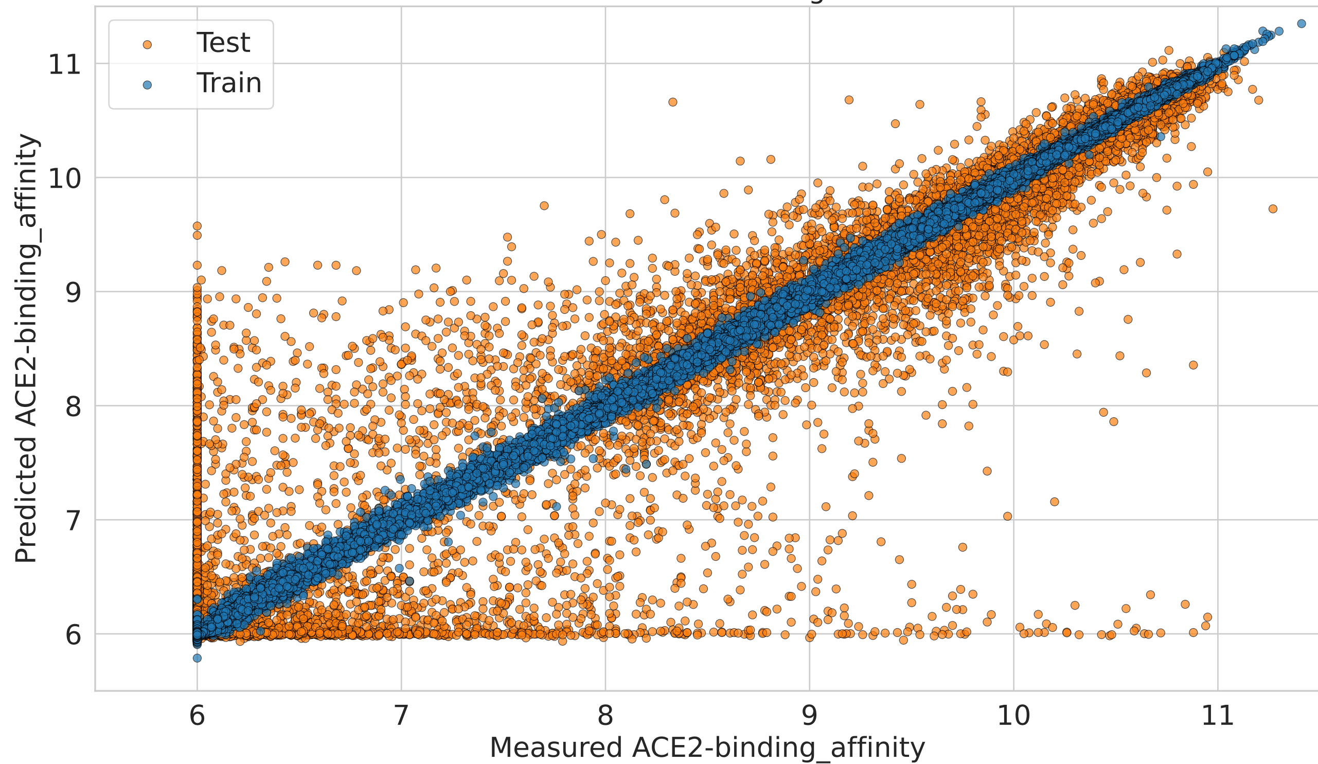
ESM-FCN Binding
