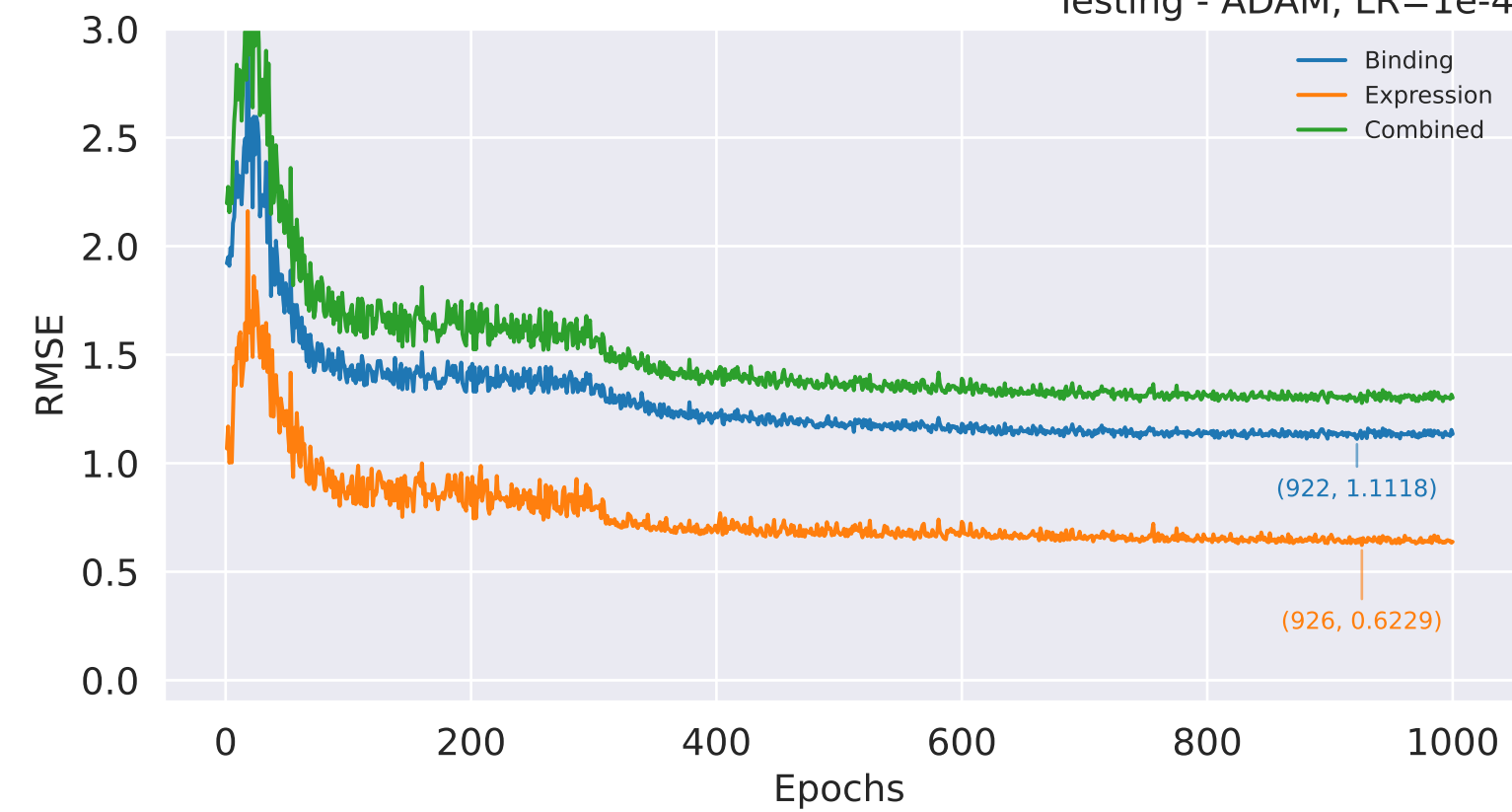
Testing - ADAM, LR=1e-4
