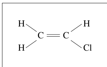
Vinyl chloride
