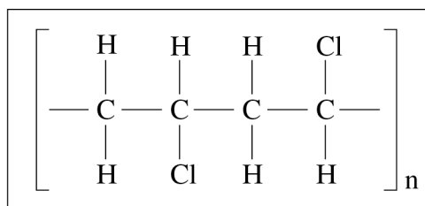
Polyvinyl chloride
