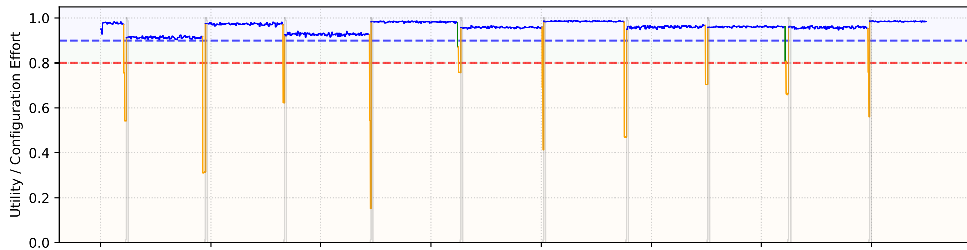
Robust
