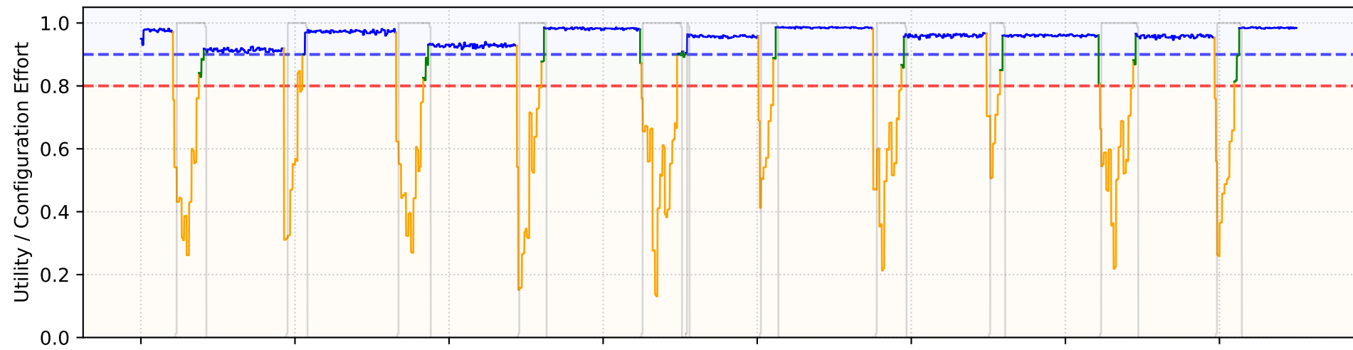
Non-Adaptive
