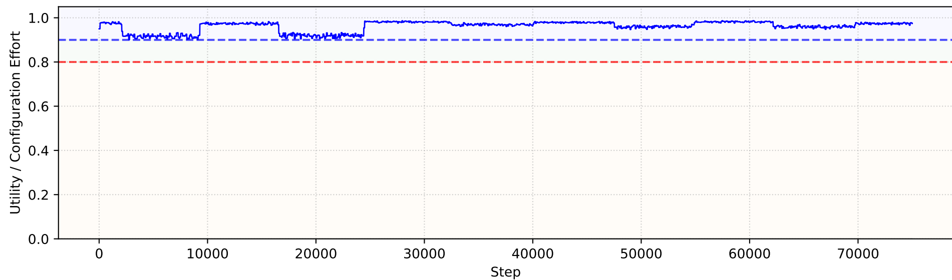
Robust
