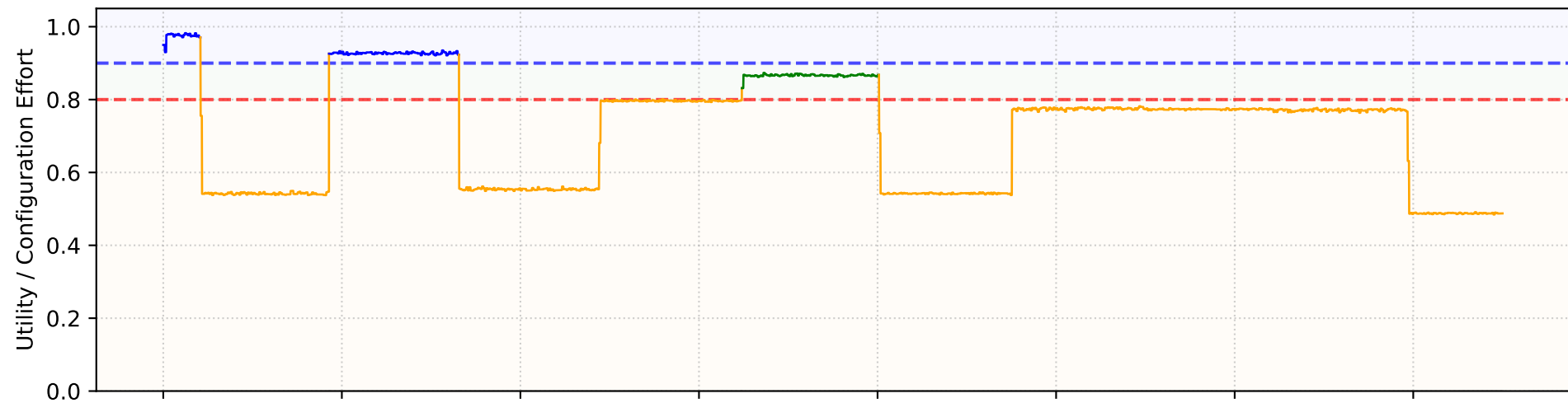
PerfectSelector
