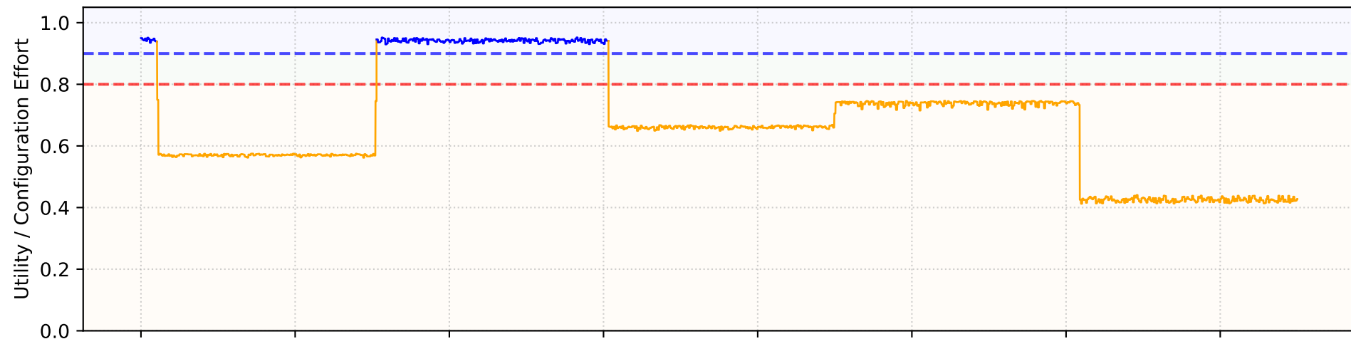
Survival-Focus
