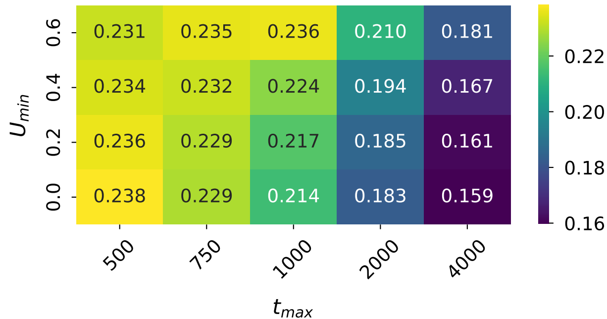
Statistical Variance
