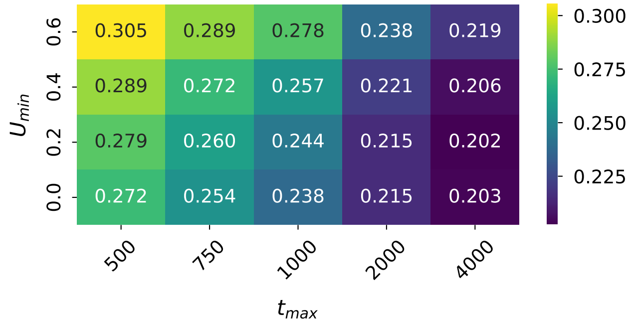
Statistical Variance
