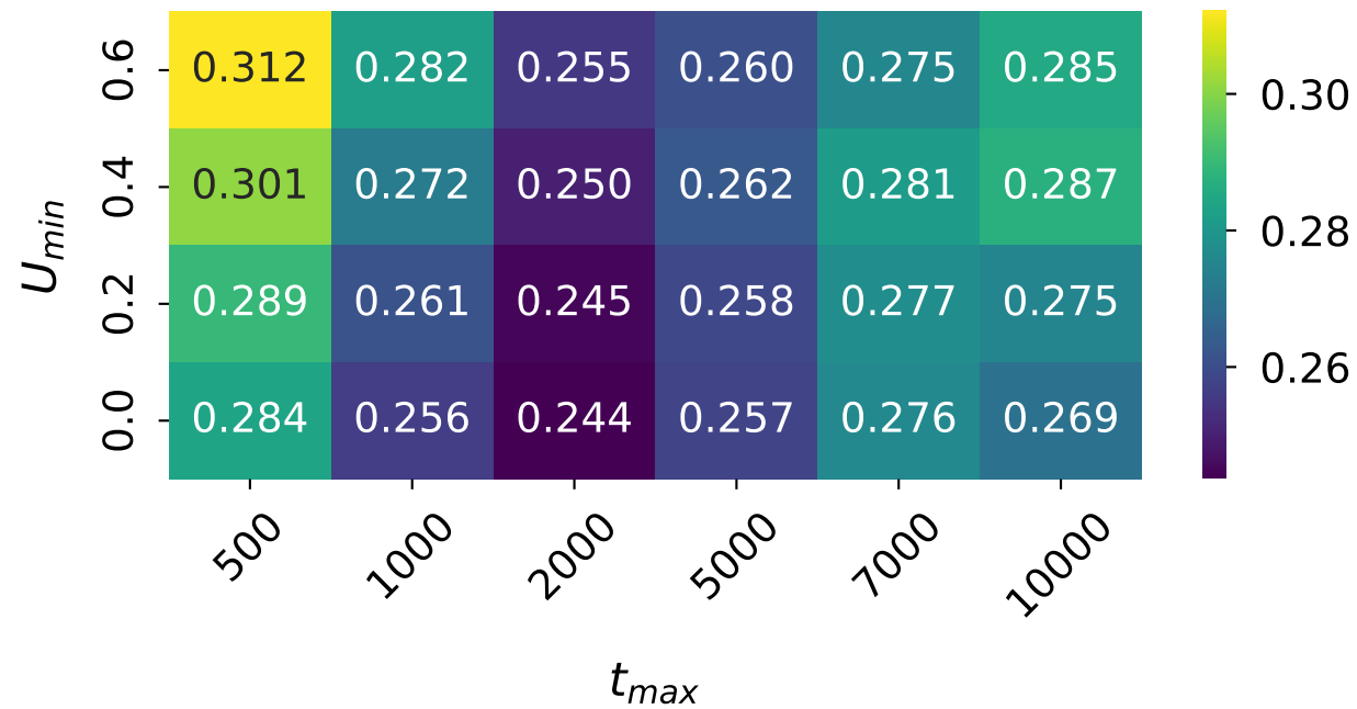
Statistical Variance
