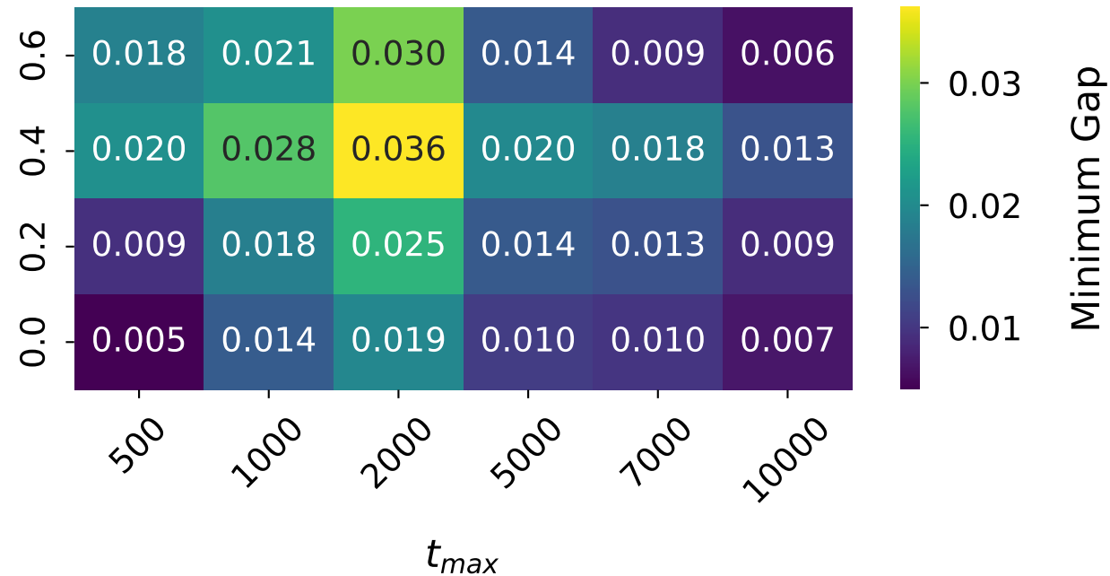
Minimum Pairwise Gap (Maximin)
