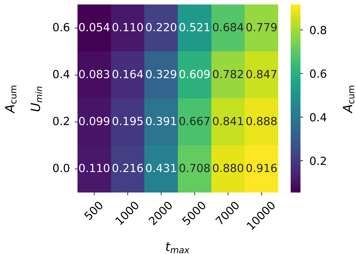
OptimisingLearner
