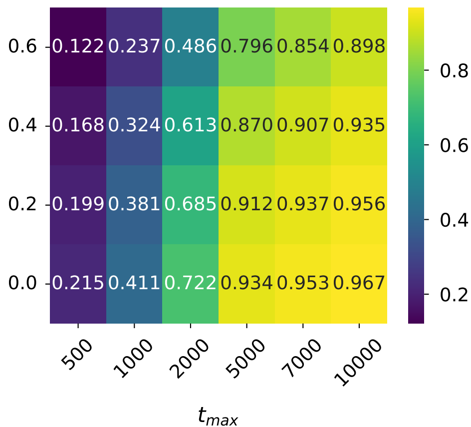
NonAdaptive
