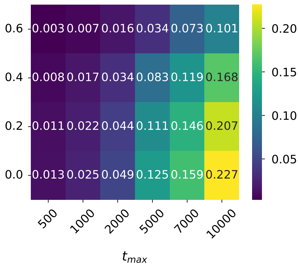
NonAdaptive
